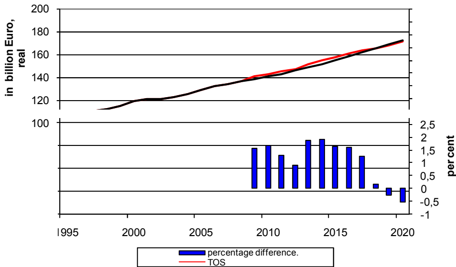
Figure 4: Households' consumption (reference and TOS)
